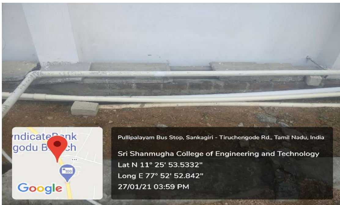
Water Distribution System from Ground Tank to Roof Tank
